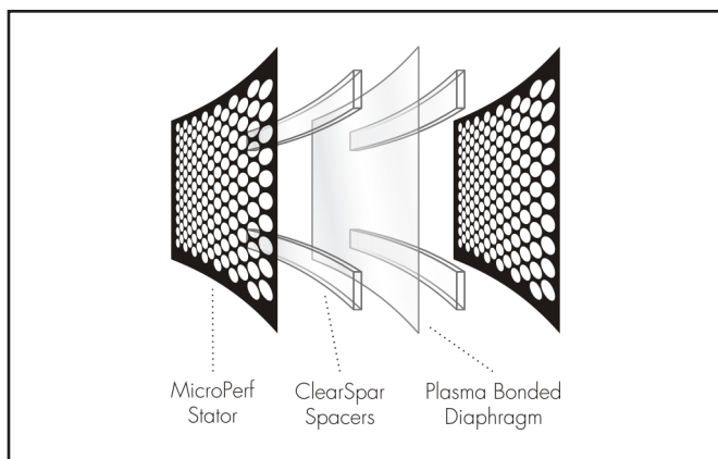
Figure 14. Cut away view of an XStat™ electrostatic transducer. Notice the simplicity due to minimal parts usage.
